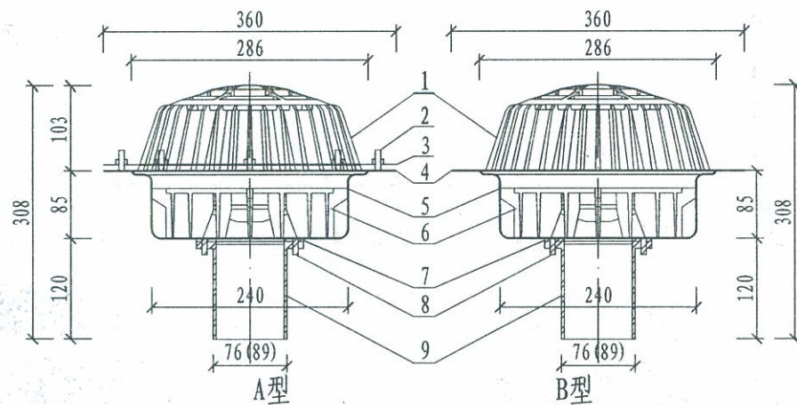
② YG75 (80)型虹吸式雨水斗
