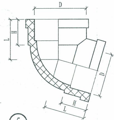
⑤ UPVC45°弯头
